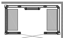
PANACEA 1709 Size: 1725 x 925 x 2090 mm Code: 96075026
