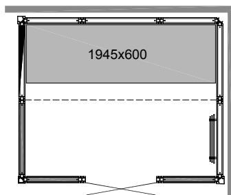
PANACEA 2117 1B Size: 2125 x 1725 x 2090 mm Code: 96075074
