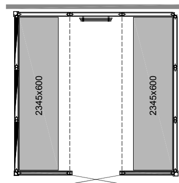
PANACEA 2525 2B Size: 2525 x 2525 x 2090 mm Code: 96075084
