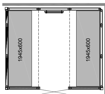
PANACEA 2521 2B Size: 2525 x 2125 x 2090 mm Code: 96075080
