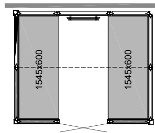
PANACEA 2117 2B Size: 2125 x 1725 x 2090 mm Code: 96075076
